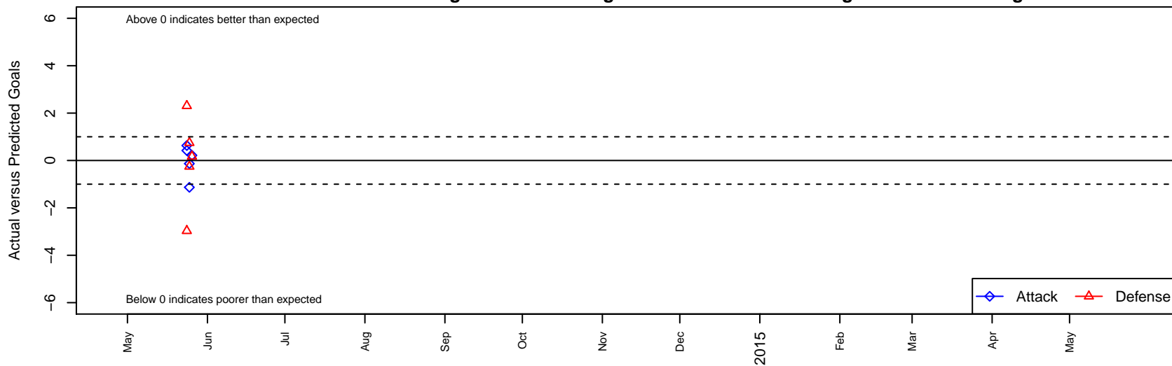
GPYSC Arsenal B00 Dots are actual minus expected GF (blue circles) and GA (red triangles). Blue line is smoothed change in attack strength. Red is smoothed change in defense strength.
